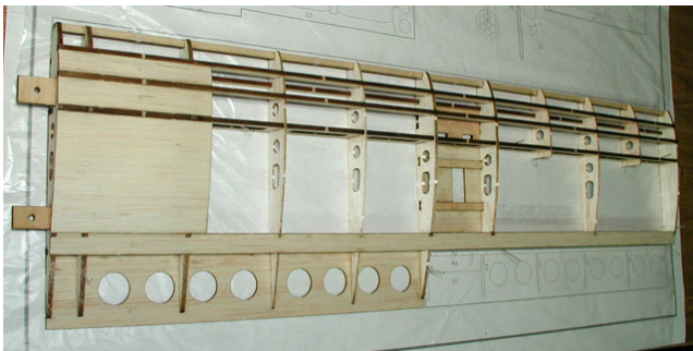
7. Glue upper trailing sheet(W23) and upper wingroot sheets(W26, W30-W31).
