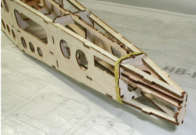
13. Temporary assemble rear left side panel(F37), top & bottom longerons(F31-F32). Install bulkhead(F34), servo trays(F35-F36, F38-F39) and Stabilizer holder(F32-F33).
