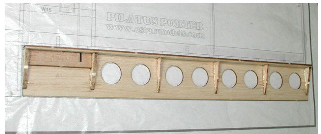
11. Pin the aileron parts(A1-A5) on the plan and glue them.
