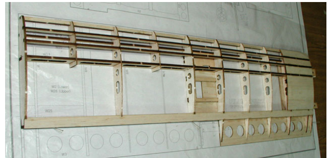
10. Assemble the other side wing.
