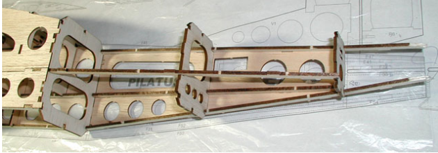
11. Temporary assemble rear right side panel(F37), rear longerons(F27-F28) and bulkheads(F29-F30).
