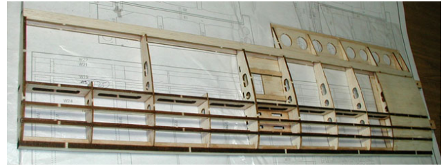
9. Glue leading edge(W22). Remove pins and apply thick CA glue at each joints for reinforcing.
