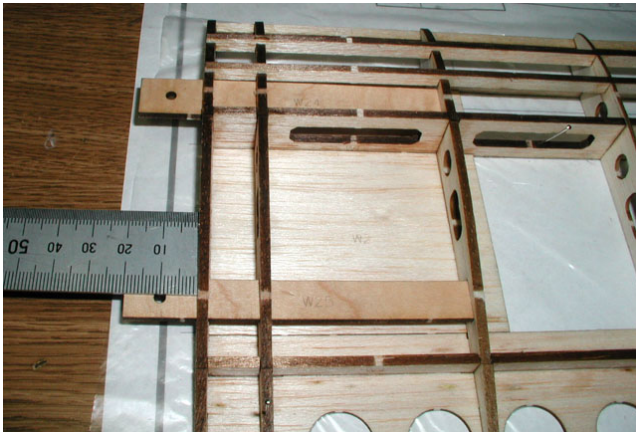
6. Glue wing joiners(W24-W25). Location of ribs are marked on the joiners.
