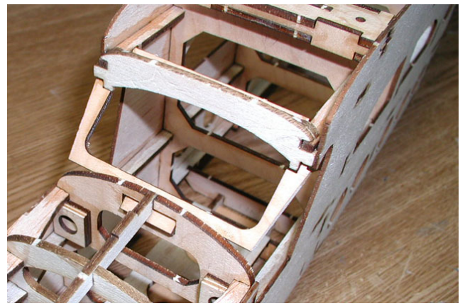
17. Glue Landing gear mounts(B12, B13) and windshield frames(F13, F15-F16).
